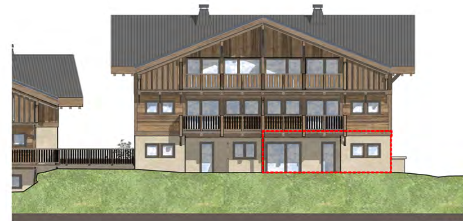
FACADE SUD
